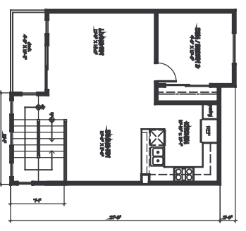
SECOND FLOOR PLAN SCALE 1/8" = 1'-0"
