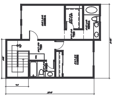
THIRD FLOOR PLAN SCALE 1/8" = 1'-0"
