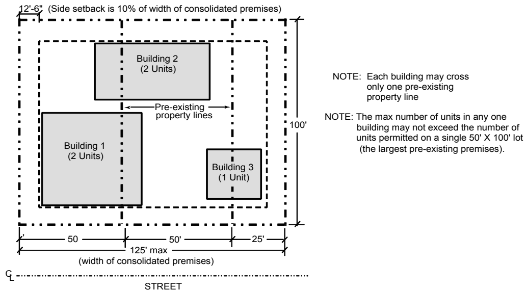
Diagram 131-04P
